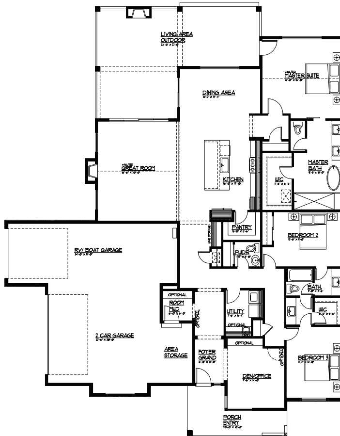
RAMBLER FLOOR PLAN
