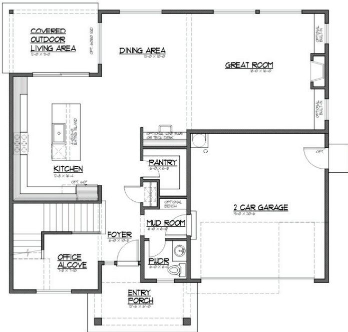
MASTER PLAN 01/24/2024
