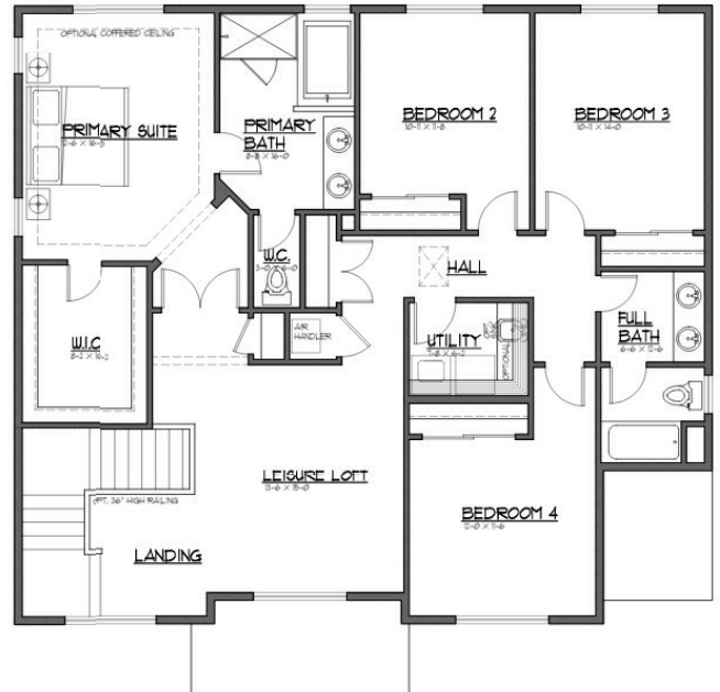
MASTER PLAN 01/24/2024
